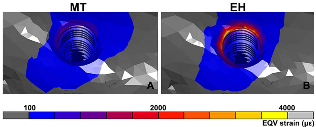
Figure 7 Occlusal view of EQV strain ( \mu\epsilon ) distribution in bone for the Morse-taper (MT) and external hexagon (EH) models, for a 640N loading. The higher strain concentration for EH connection is visible.
