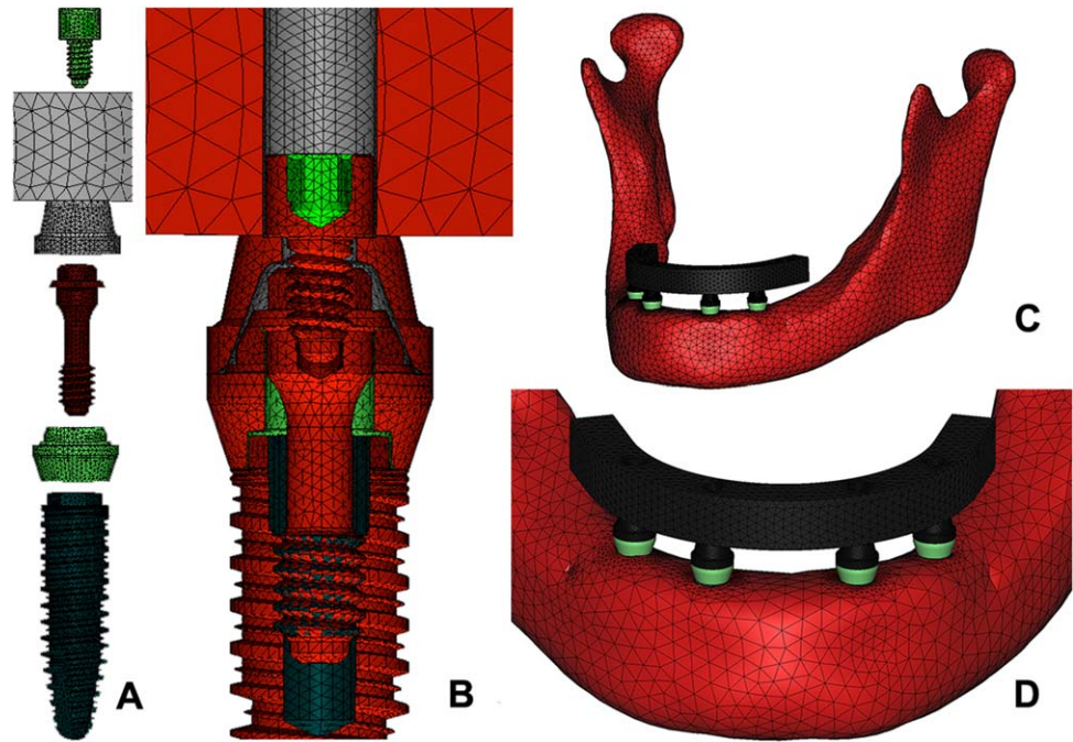
Figure 2 A – external hexagon implant system 3D meshes; B – final positioning of implant system (3D FE models are shown as sectional view); C – final finite element model, lateral view; D – final finite element model, frontal view.
